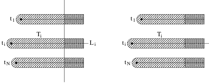
Fig. 17. On the left the pair (S_R^+ \cup_i T_i \setminus A_R, S_R^+ \setminus A_R) , on the right the pair (\sqcup_i T_i, \sqcup_i (S_R^+ \cap T_i)) .
